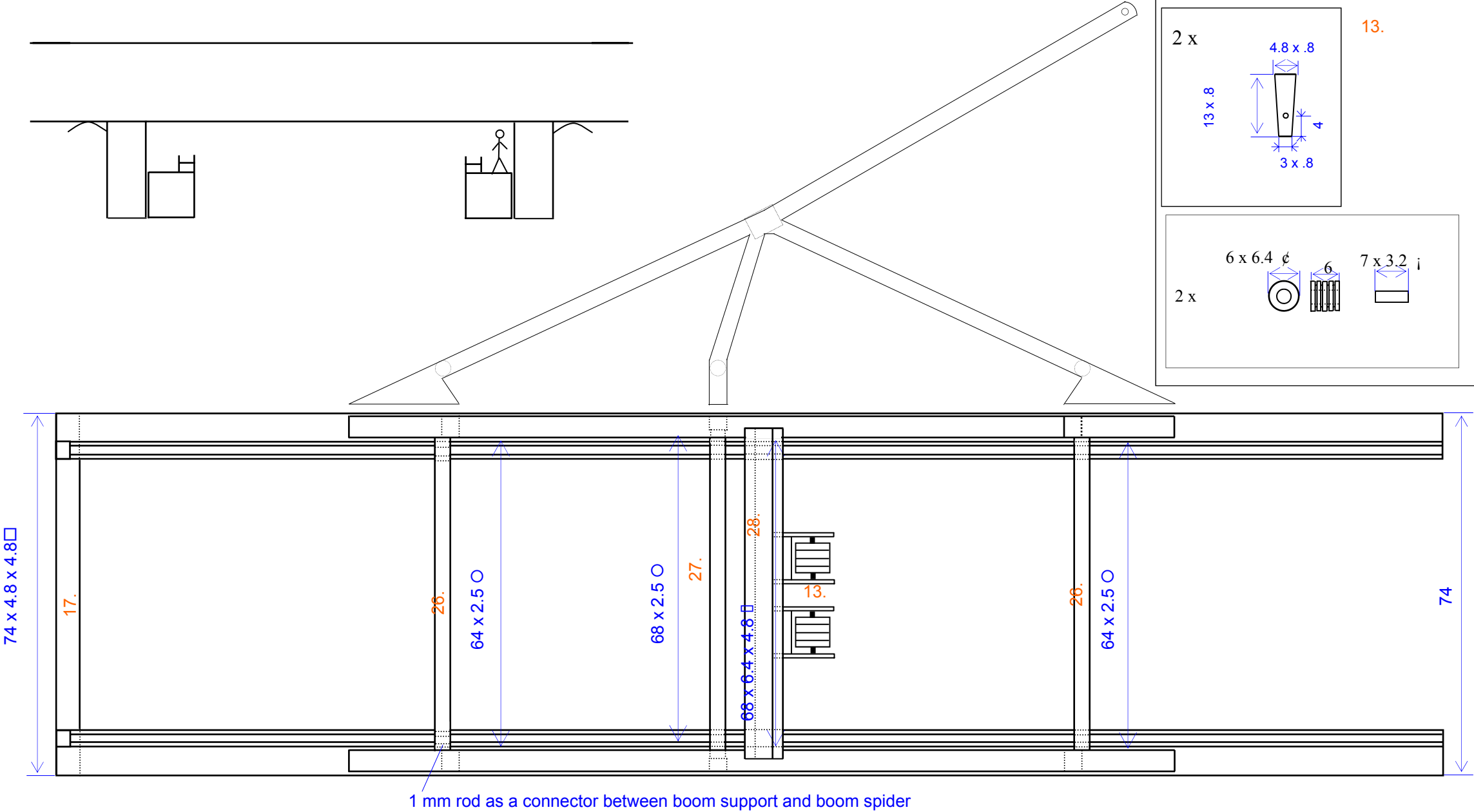
Kalmar Crane, Boom top view
